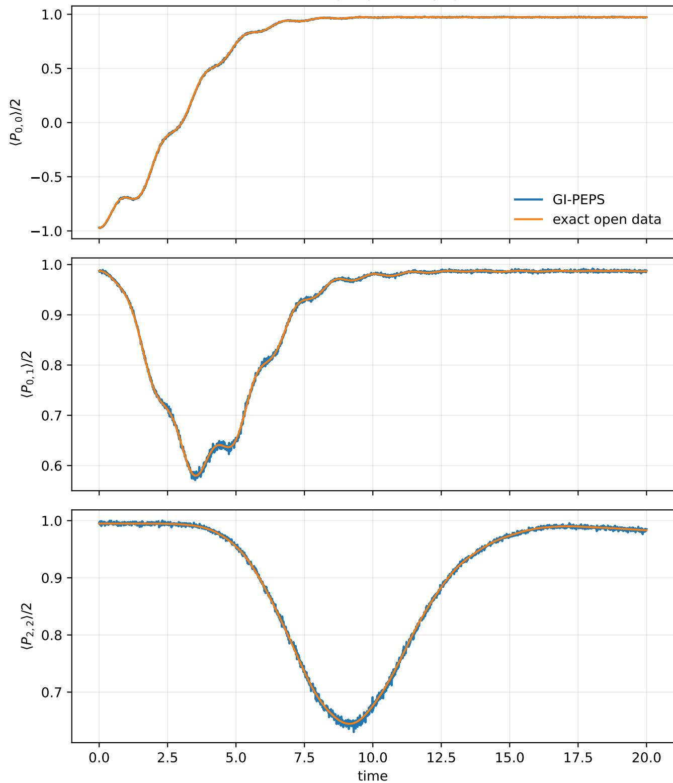
(a) 6 \times 6 Z_2 gauge theory, g = 0.1
