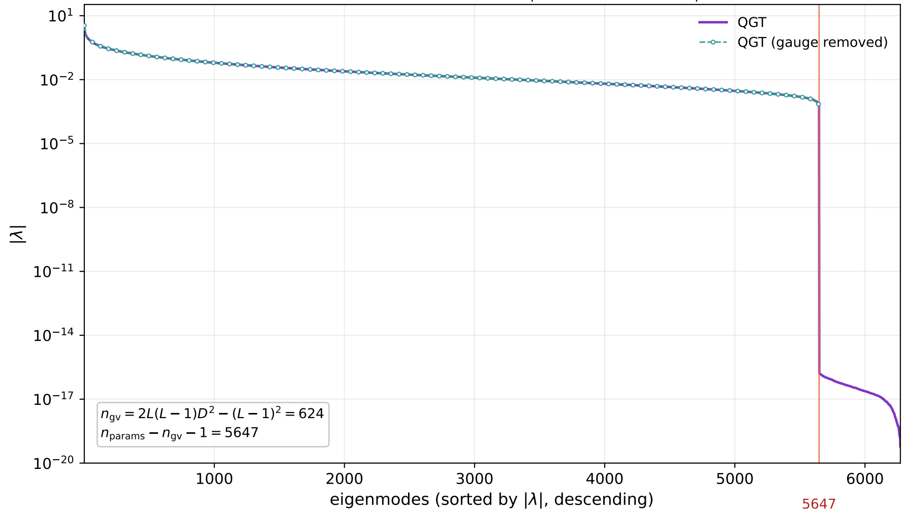
5 × 5 D = 4 Exact PEPS QGT spectrum ( n_{\text{params}} = 6272 , n_{\text{samples}} = 20480 )
