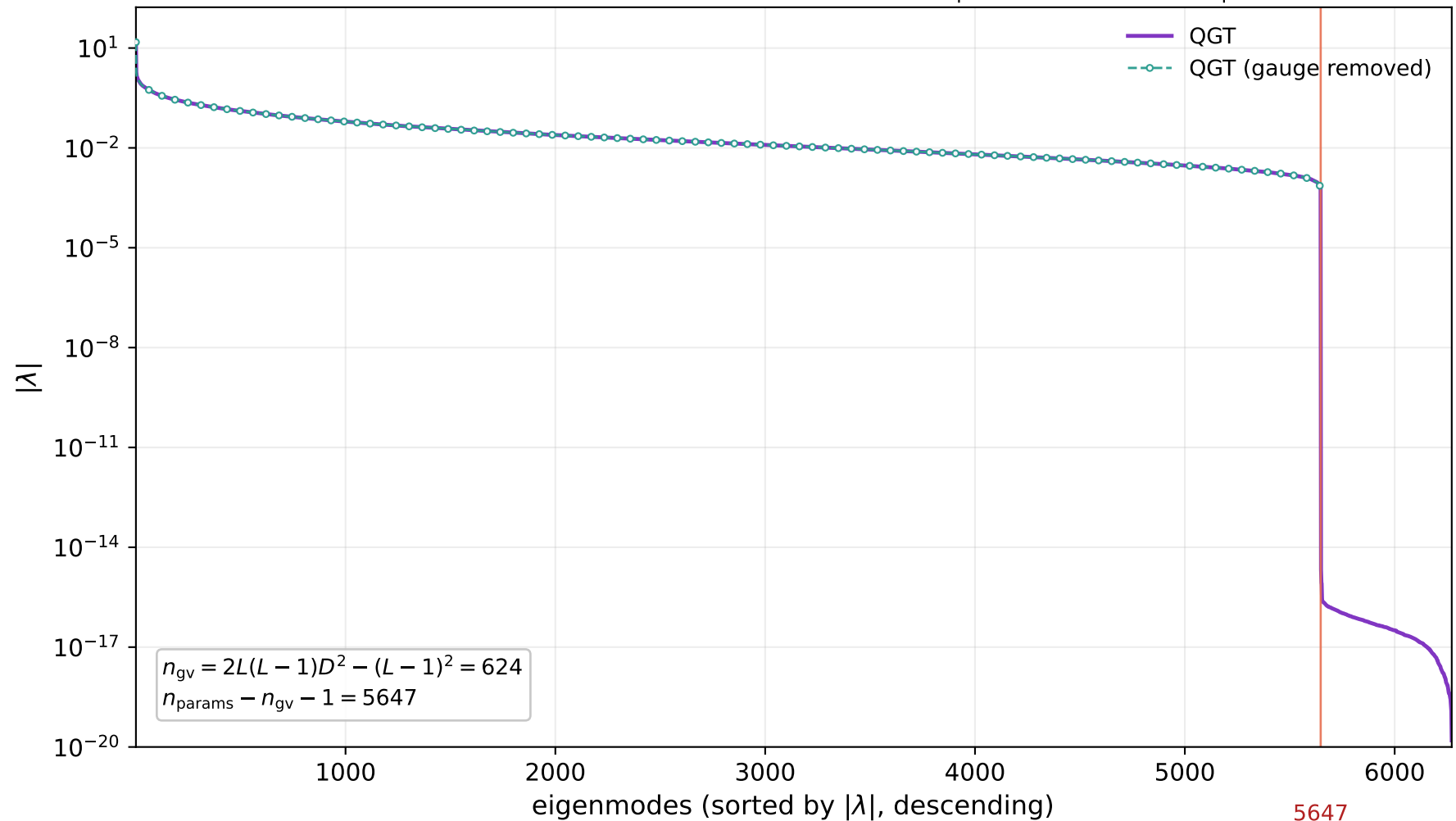
5 × 5 D = 4 Variational( D_c = 16 ) PEPS QGT spectrum ( n_{\text{params}} = 6272 , n_{\text{samples}} = 20480 )
