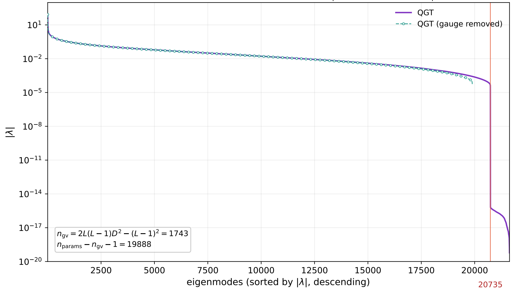
8 \times 8 D = 4 Variational( D_c = 16 ) PEPS QGT spectrum ( n_{\text{params}} = 21632 , n_{\text{samples}} = 24000 )
