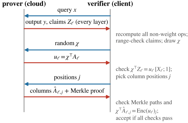
Figure 2: One query of our protocol (committed weights).
