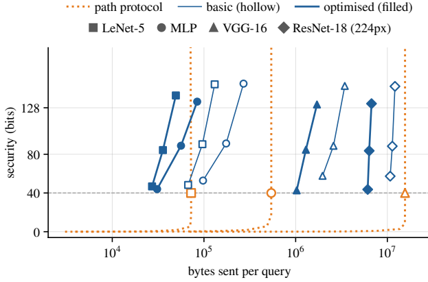
Figure 3: Security against bytes sent: our proofs buy far more security per byte than the paths
