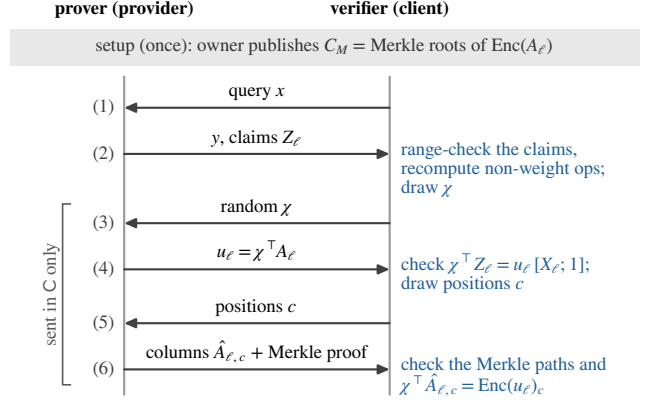
Figure 2: One query in setting C: each value is fixed before the randomness that tests it
