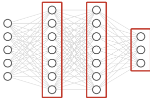
(c) Our defence: check every layer at once \chi^\top Z \stackrel{?}{=} (\chi^\top W) X for every layer
