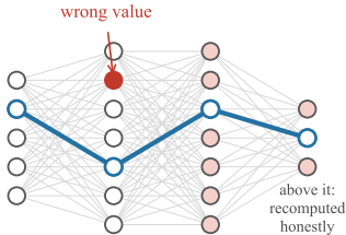
(b) Our attack: change one neuron
