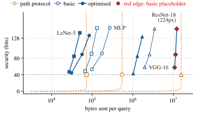
Figure 3: Security against bytes sent per query, in bits: -\log_2 of the probability that a wrong output is accepted (paths: the single-neuron attack; ours: the proven bound at \lambda=40, 80, 128 ; hollow: basic; shape: model). The paths reach 40 bits only by opening the whole model and trace (vertical lines).
