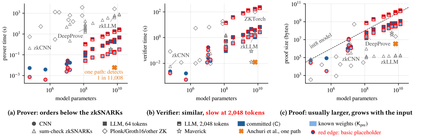
Figure 4: Cost against model size: the optimised protocol (blue; verifier on 8 CPU threads) and published systems as reported on their own hardware (grey; orange: one path of [2]). Table 5 compares them on matched models.
