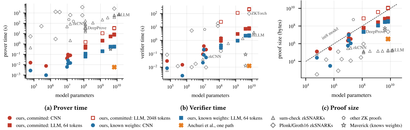
Figure 4: Cost against model size.
