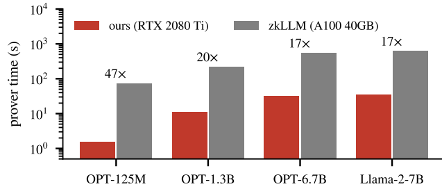
Figure 5: Prover time at 2,048 tokens: ours against zkLLM.
