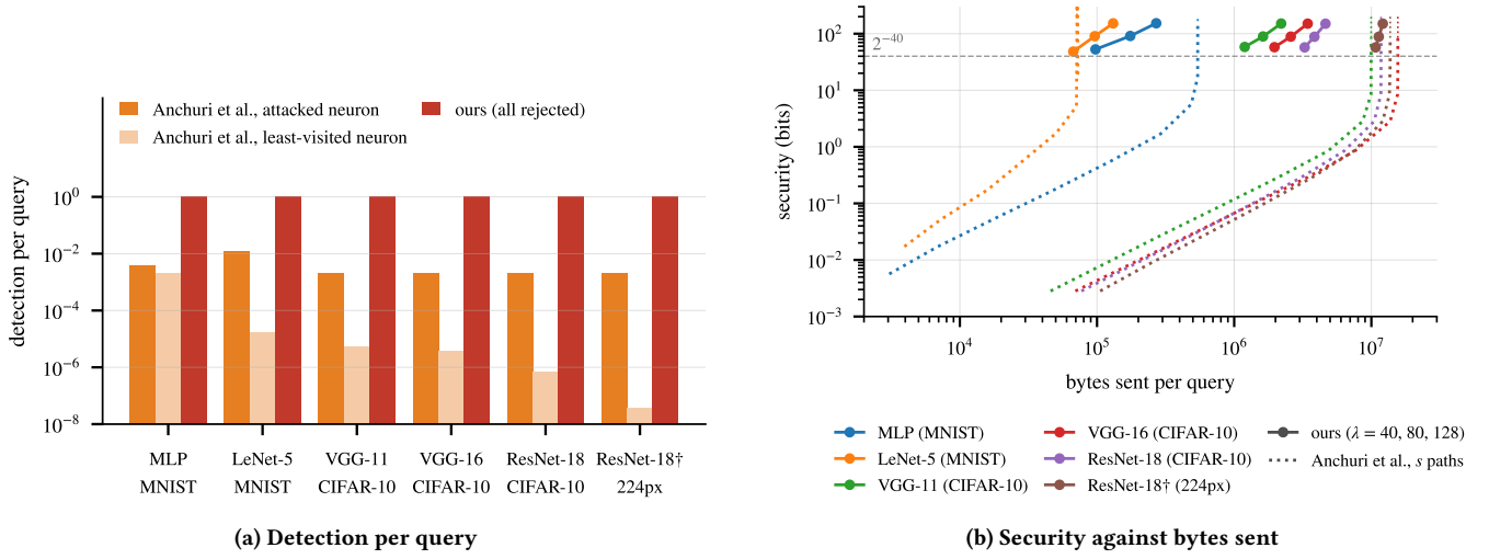
Figure 3: Catching the single-neuron attack.
