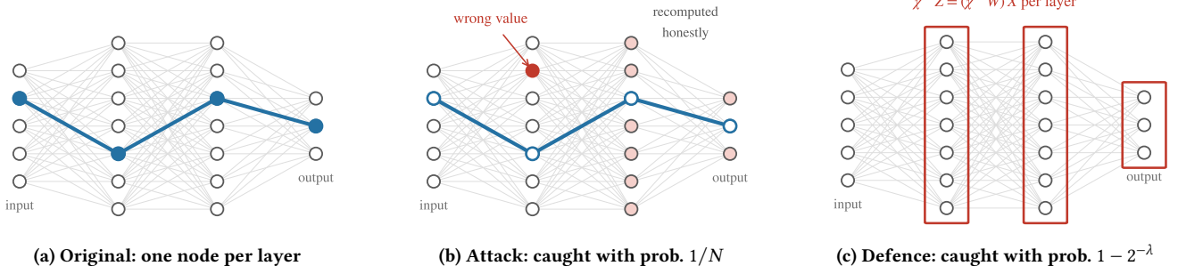
Figure 1: Checking one path versus checking every layer.
