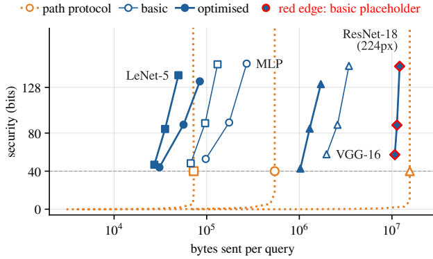
Figure 3: Security against bytes sent: our proofs buy far more security per byte than the paths
