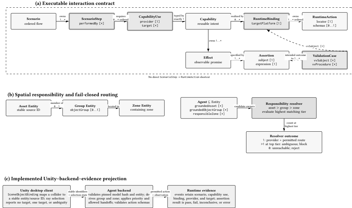
Fig. 2. The compact FunctionalMLDS contract and its implementation mapping. A scenario step reaches a runtime action only through an explicitly provided capability use, capability, and binding. Spatial responsibility is resolved at the highest matching tier—asset before object group before zone—and ambiguity at that tier blocks execution. Stable model identifiers connect the Unity selection, backend routing, and structured assertion evidence.
