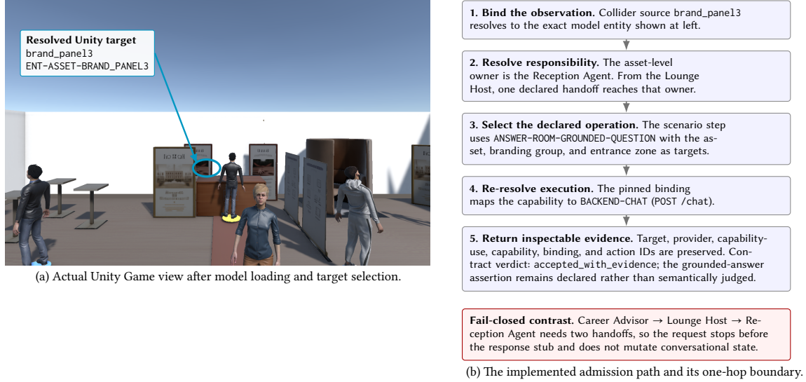
Fig. 1. Concrete model-grounded interaction in the Steinpilz scene. The left image is a reproducible capture from the implemented Unity project; the cyan marker and label are paper annotations placed at the collider center logged by the capture runner, not additional visitor controls. The right side follows the exact success and rejection cases reported in the benchmark.
