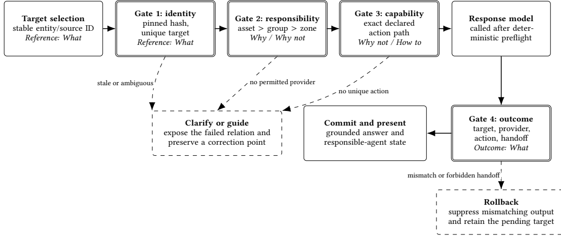
Fig. 1. Fail-closed admission path organized by intelligibility question. Reference, responsibility, and capability checks precede generation; outcome evidence determines whether the response is presented or rolled back.
