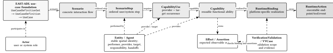
Fig. 2. Selected core of FunctionalMLDS. The EAST-ADL use-case foundation is extended with explicit scenario flow, spatial entities and agents, scenario-specific capability uses, executable runtime mappings, and observation-oriented validation. Attributes and secondary associations are omitted for readability.
