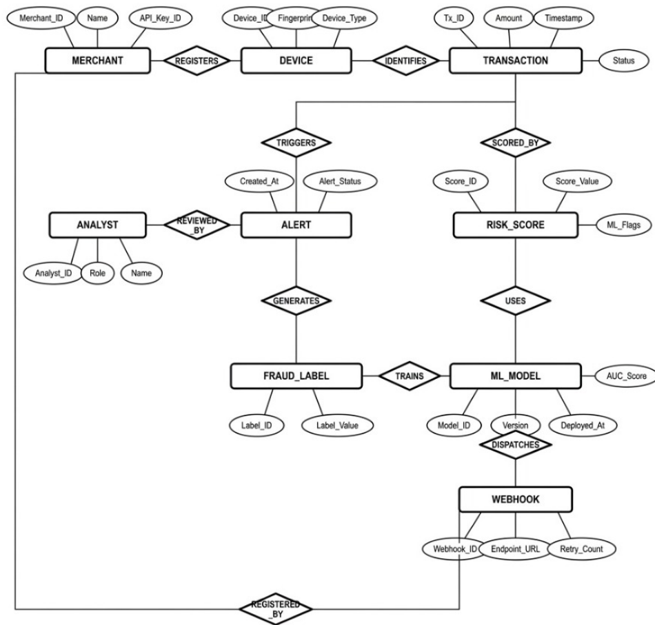
Figure 5: Entity-Relationship (ER) diagram of the planned database schema.
