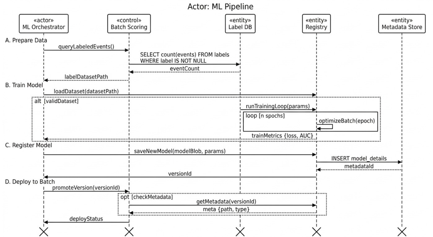
Figure 4: Sequence diagram 3: additional sequence flow.
