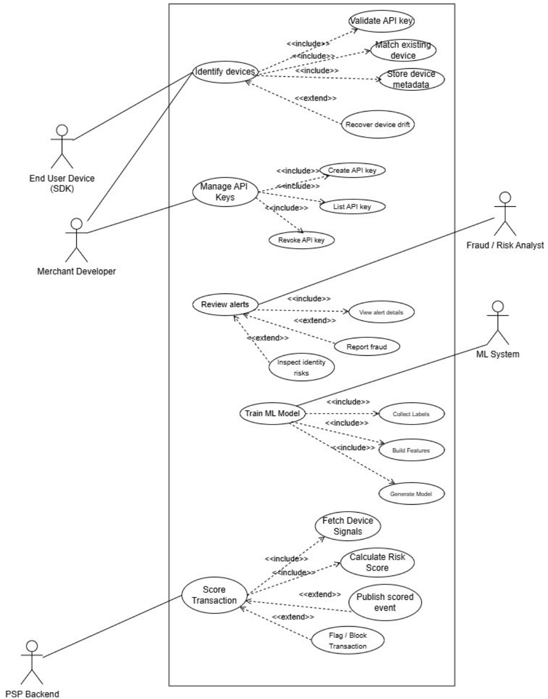
Figure 1: Updated use case diagram (PSP Backend, Web SDK, Fraud Analyst).
