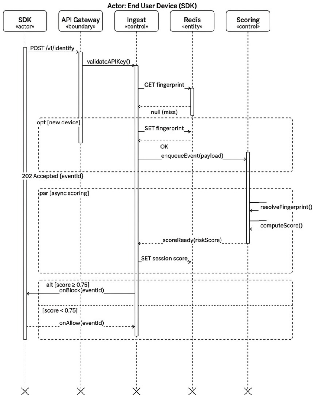
Figure 2: Sequence diagram 1: device identification flow.
