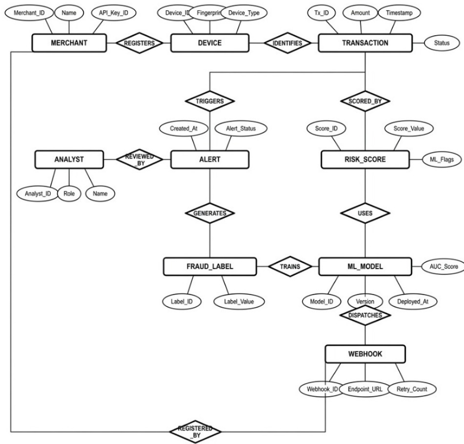
Figure 6: Entity-Relationship (ER) Diagram of the database schema.
