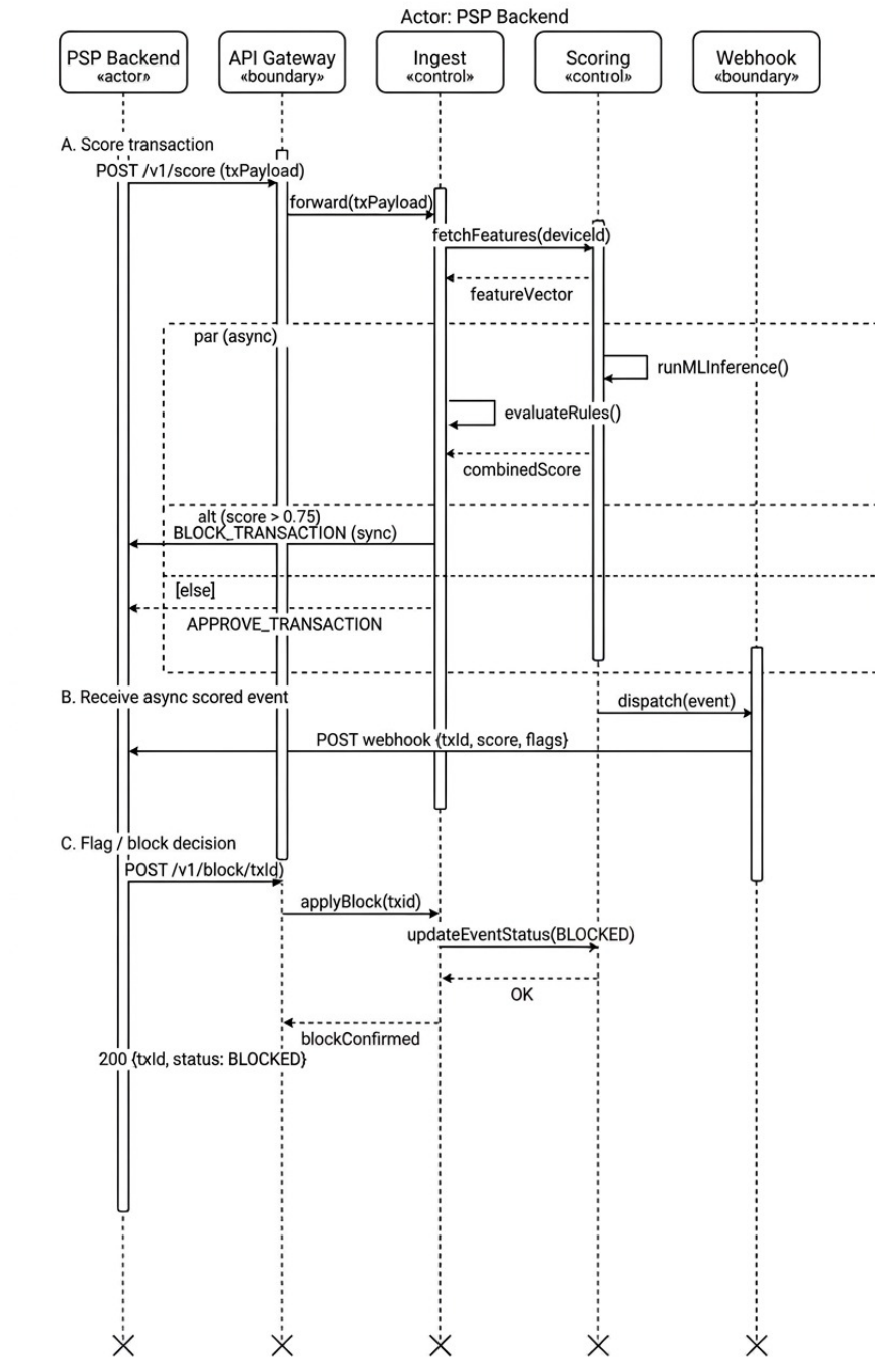
Figure 5: Sequence diagram 4: additional sequence flow.
