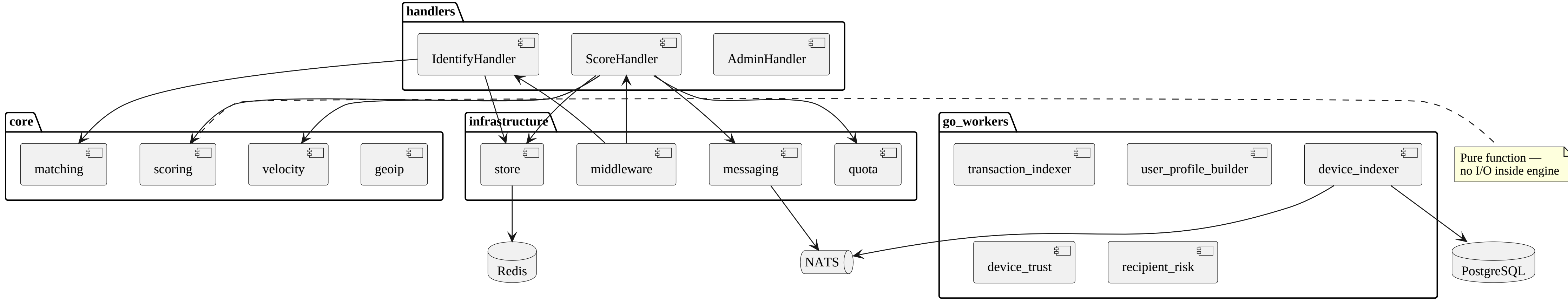
Flint Secure — Component Diagram (Go API)
