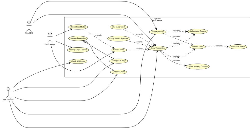
Figure 1: Use case diagram with association, include, extend, and generalization.
