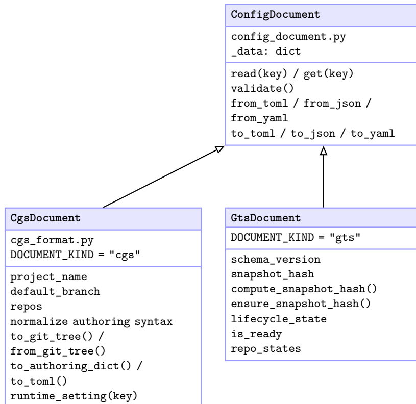
Figure 3.8: Document class hierarchy. ConfigDocument is the abstract base; each concrete subclass parses and validates one file format.
