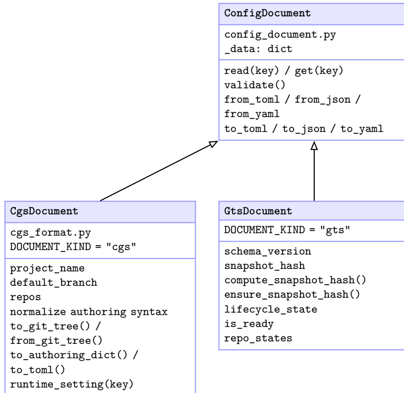
Figure 8: Document class hierarchy. ConfigDocument is the abstract base; each concrete subclass parses and validates one file format.
