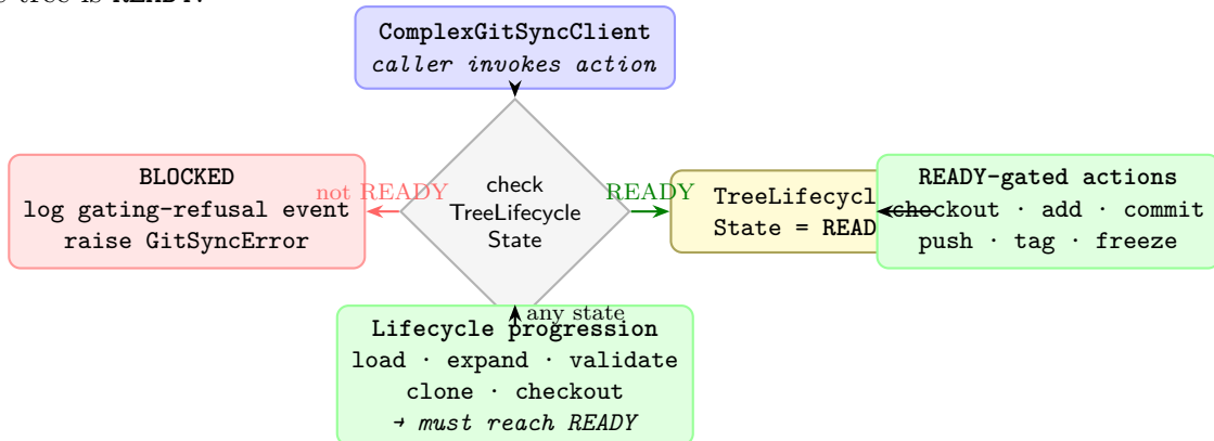
Figure 5: Client state-gating: the Client reads TreeLifecycleState before delegating to an action. READY-gated actions (checkout, add, commit, push, tag, freeze) are blocked unless the tree is READY.
