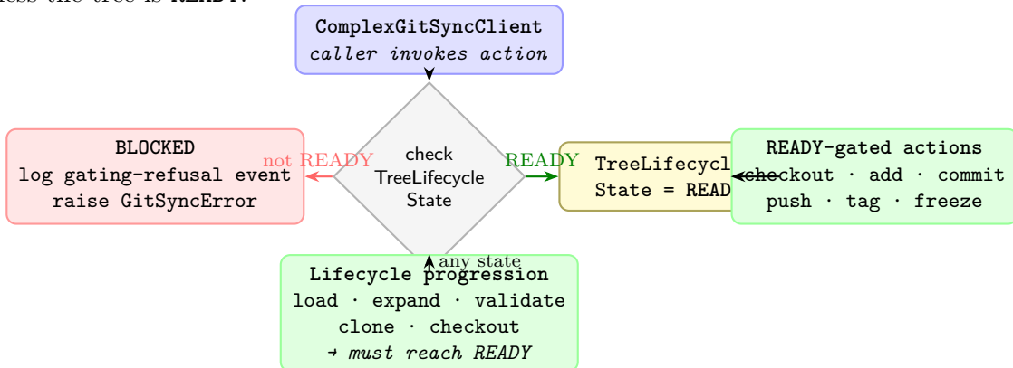
Figure 5: Client state-gating: the Client reads TreeLifecycleState before delegating to an action. READY -gated actions ( checkout , add , commit , push , tag , release freeze ) are blocked unless the tree is READY .
