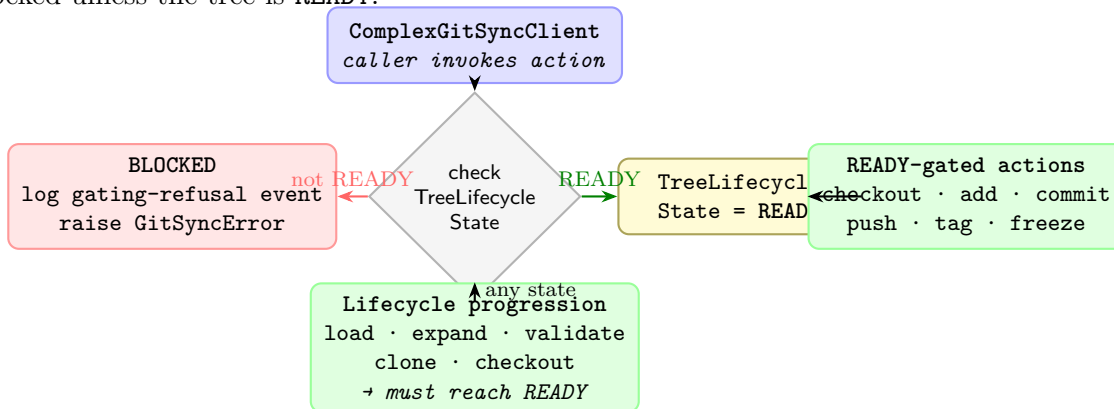
Figure 3.5: Client state-gating: the Client reads TreeLifecycleState before delegating to an action. READY -gated actions ( checkout , add , commit , push , tag , freeze-release ) are blocked unless the tree is READY .
