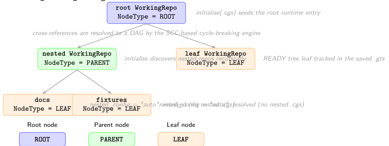
Figure 3.3: WorkingGitTree is a parent-leaf graph of WorkingRepo nodes. Root and parent nodes own nested .cgs files discovered during initialise , bootstrap or discover_nested_configs .
