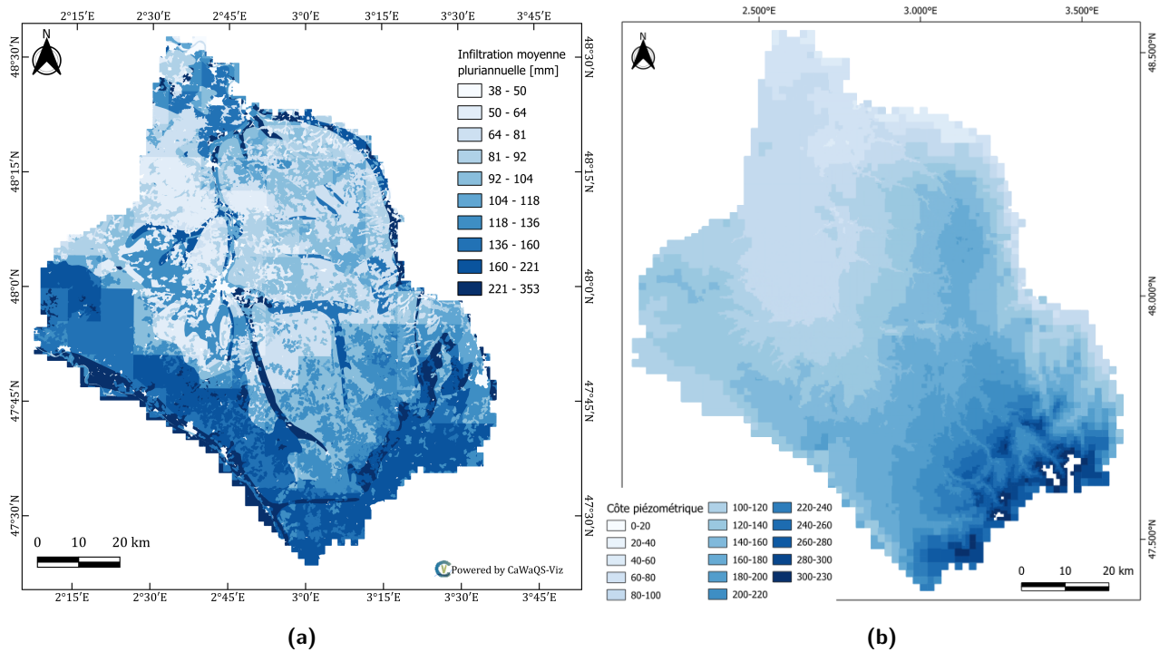
Figure 3.7: Spatialisation of mean inter-annual infiltration flux [mm] (a) and piezometry [mNGF] (b) simulated at the scale of the Loing hydrosystem
