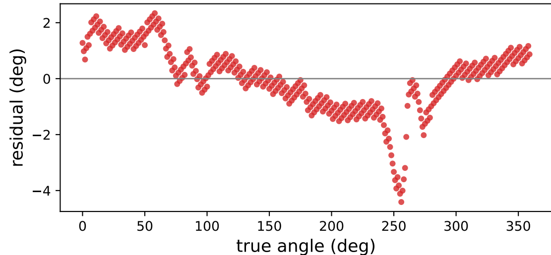
Factor recovery residual
