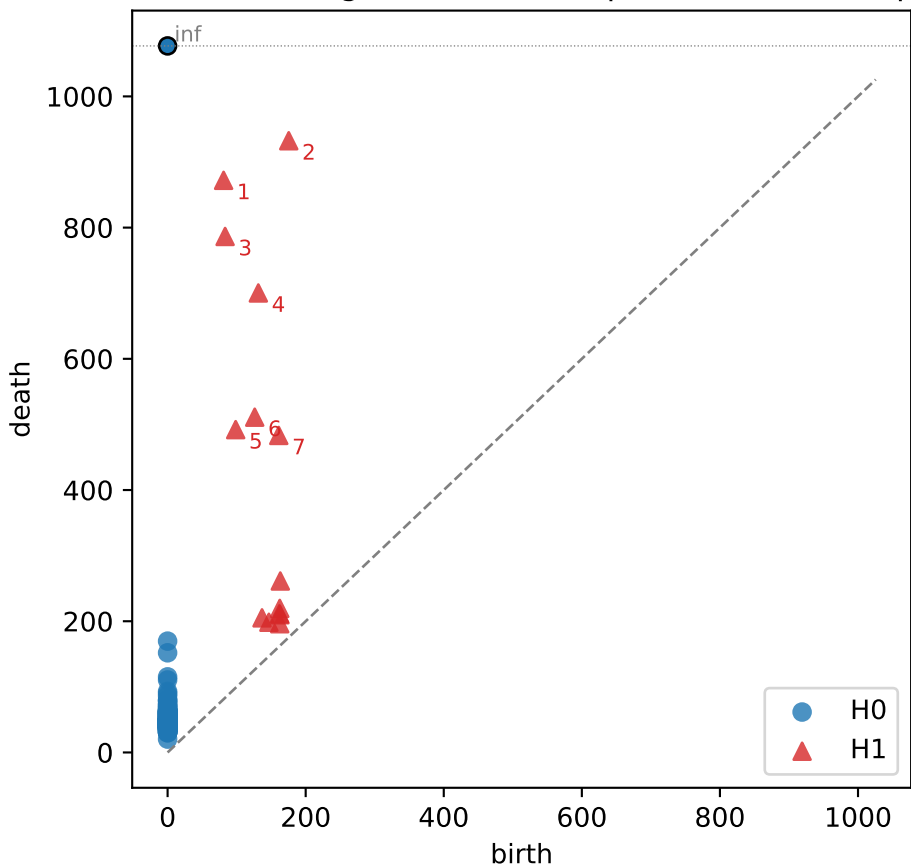
Persistence diagram (H0 = components, H1 = loops)
