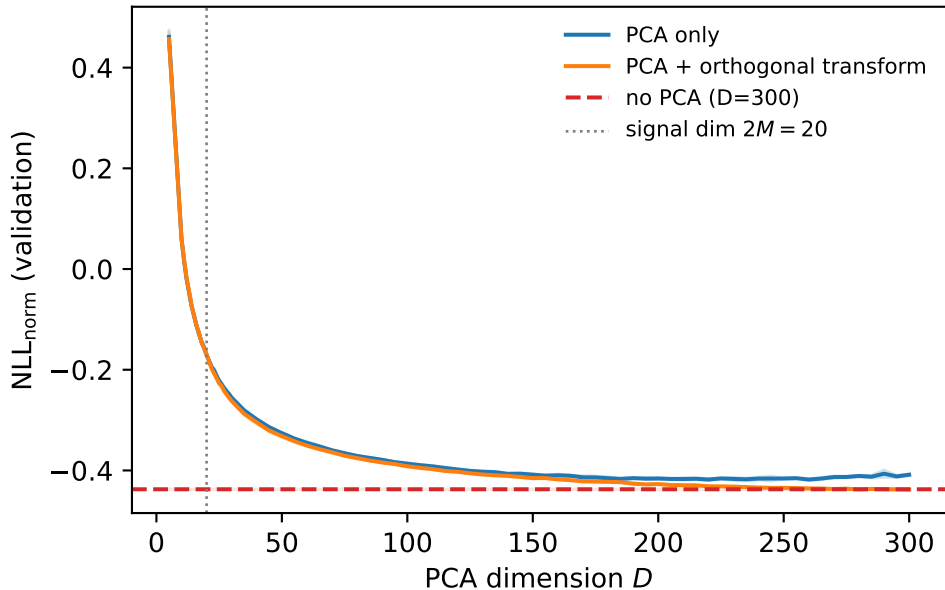
Density fit vs. PCA dimension
