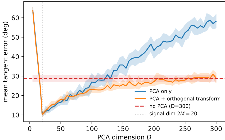
Tangent recovery vs. PCA dimension
