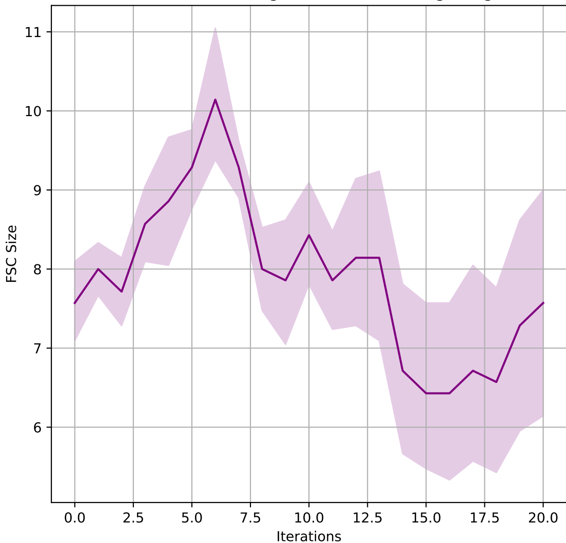
FSC Size for .moving-obstacles-6-3 using Alergia
