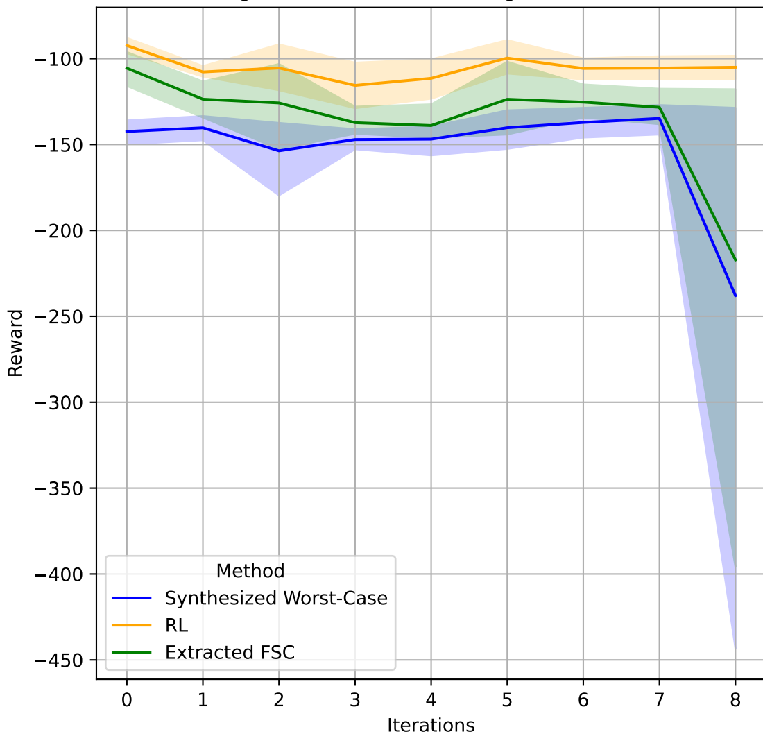
Convergence Curves for moving-obstacles-6-3-xl
