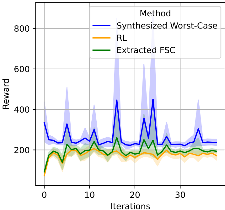
Convergence Curves for obstacles-10-5
