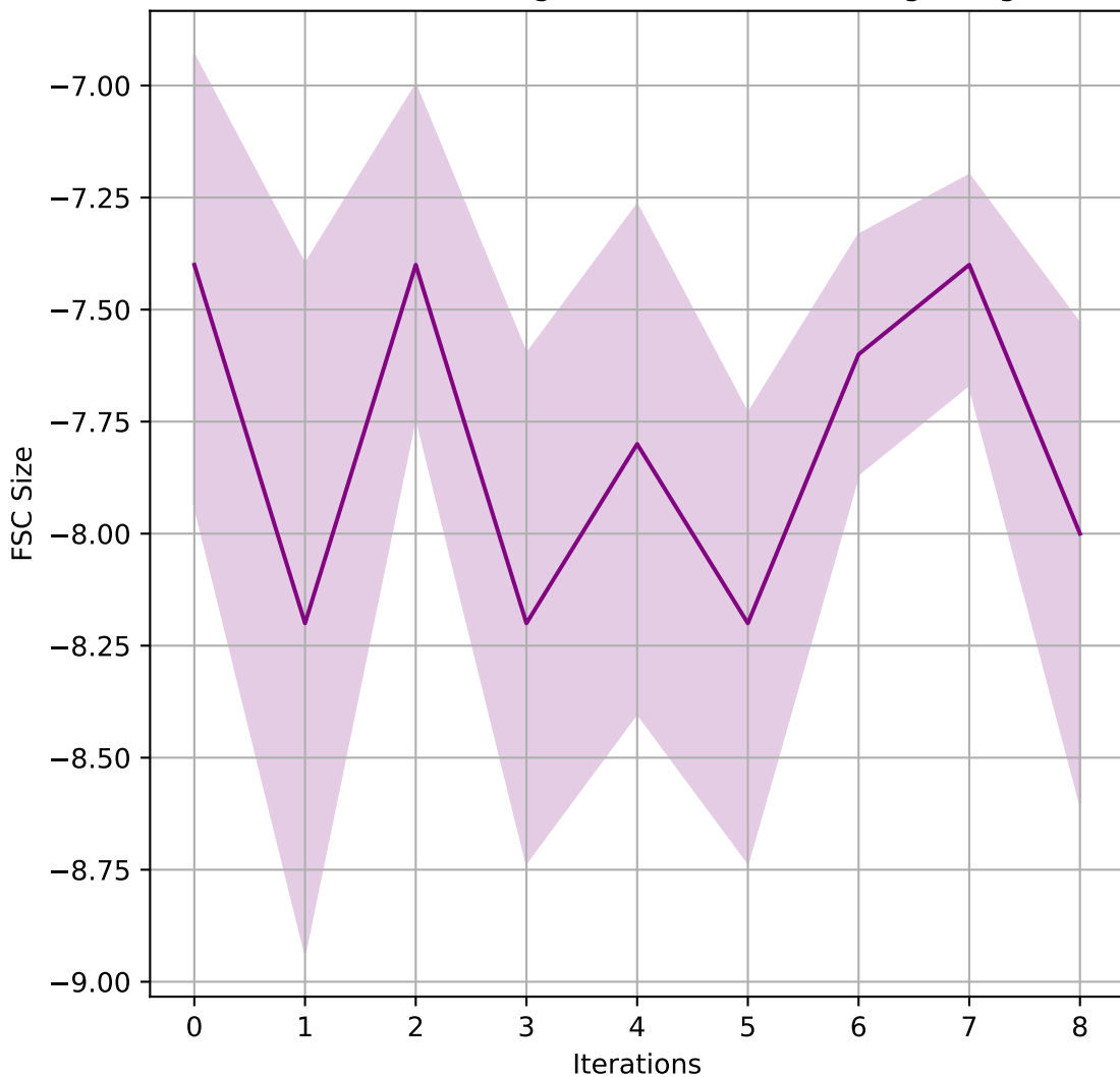
FSC Size for moving-obstacles-6-3-xl using Alergia
