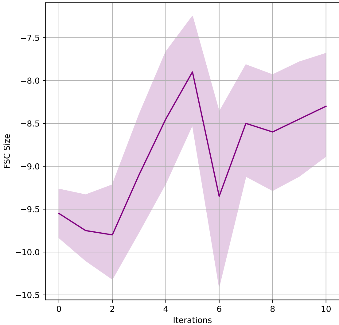
Alergia moving-obstacles-large-fam FSC Sizes
