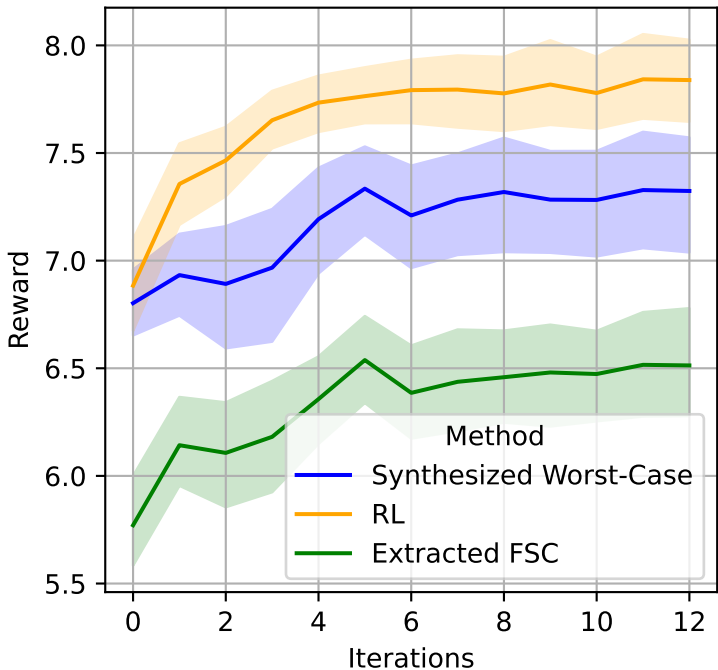
Convergence Curves for maze-10
