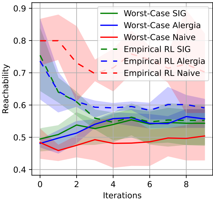
Convergence Curves for Drone
