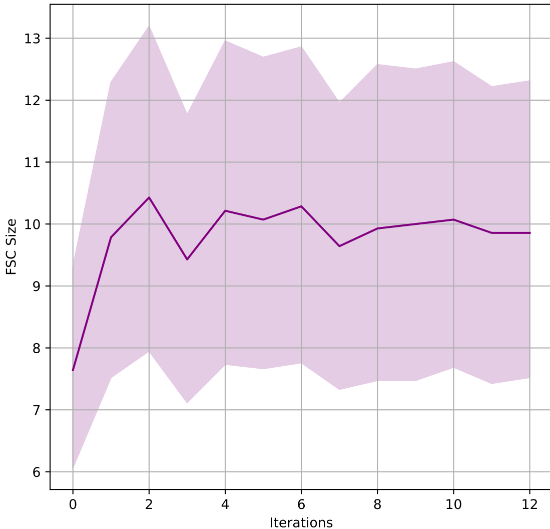
FSC Size for maze-10 using Alergia
