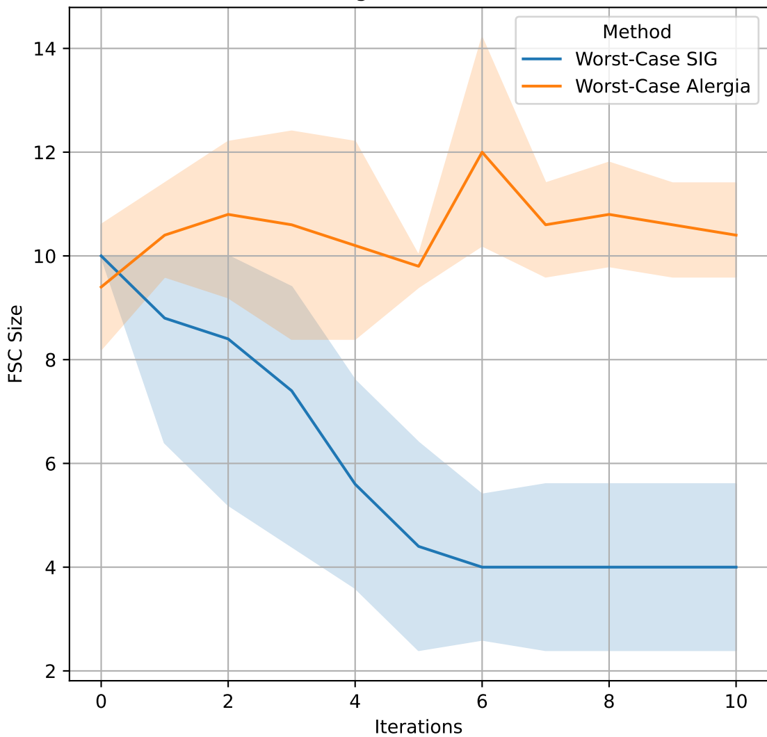
SIG moving-obstacles FSC Sizes
