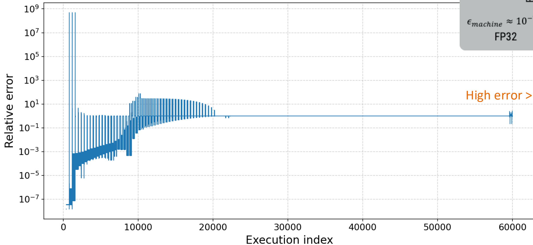
FPChecker relative error series for line 90
