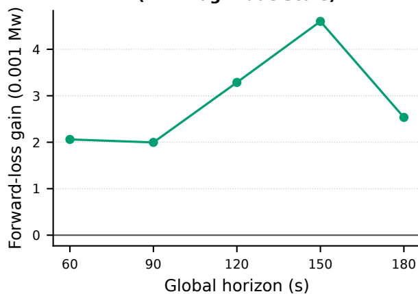
External online gain (millimagnitude scale)
