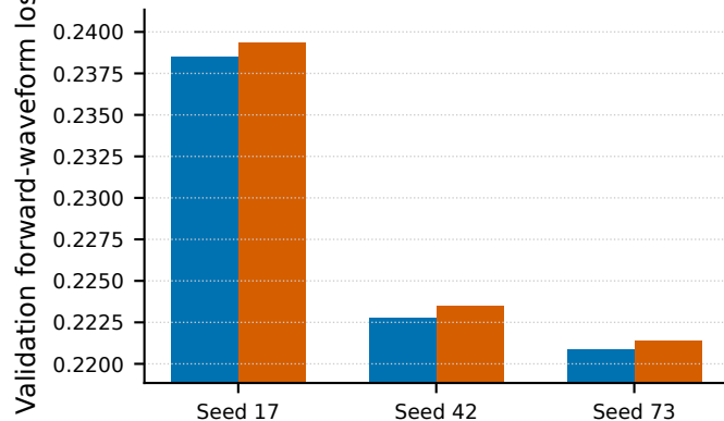
Forward-waveform mismatch (lower with full loss)
