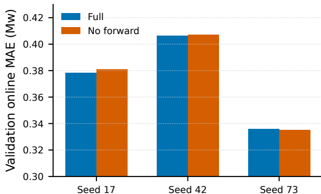
Validation online MAE (seed-dependent effect)
