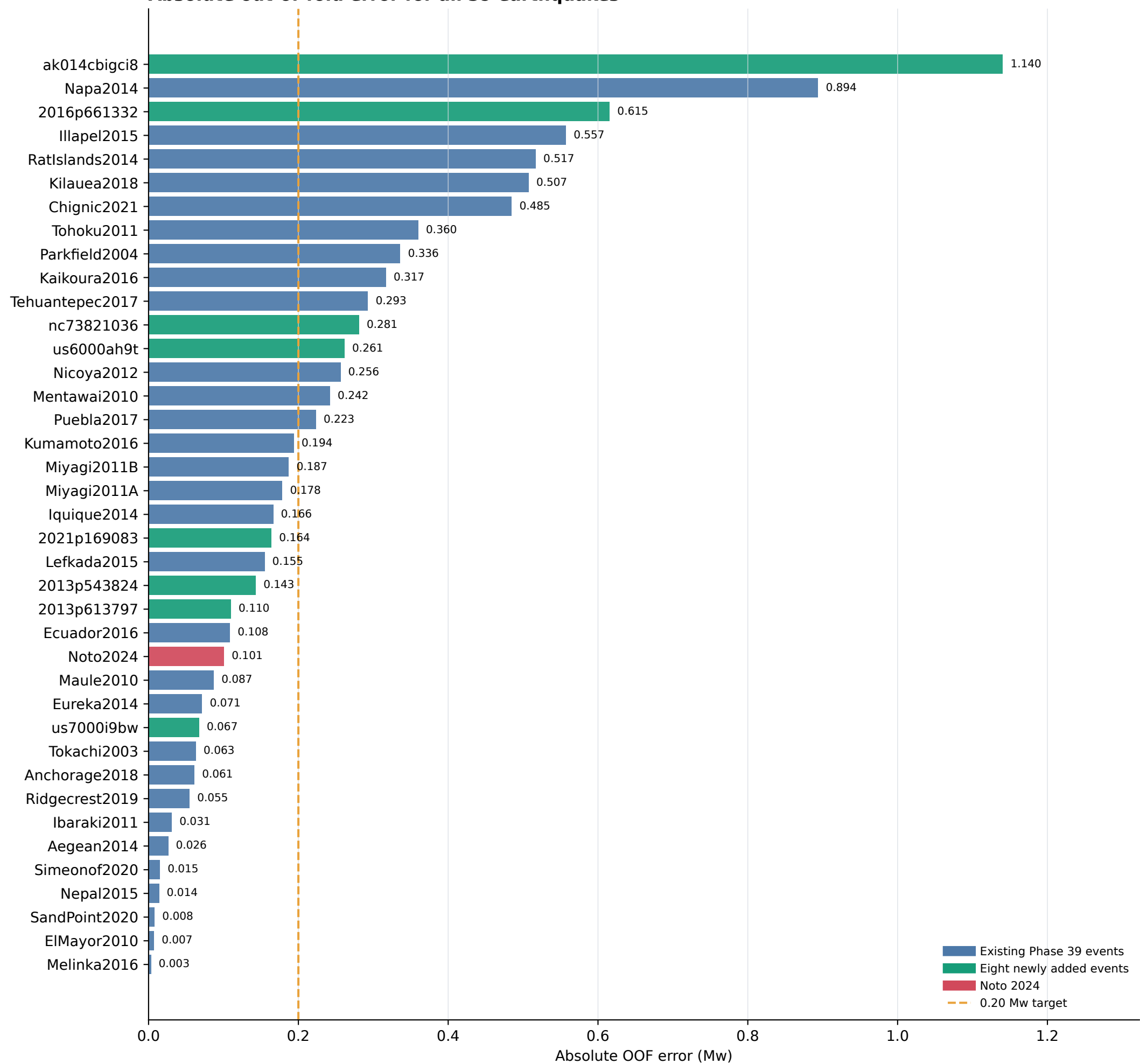
Absolute out-of-fold error for all 39 earthquakes
