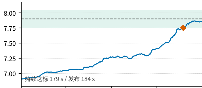
Kodiak 2018 M7.9 | 参考 7.9 | 200 s 预测 7.860
