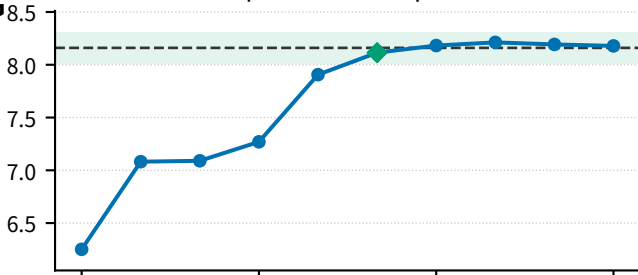
G Tokachi2003 | 目录 Mw 8.16 | n20/n200=6/34
