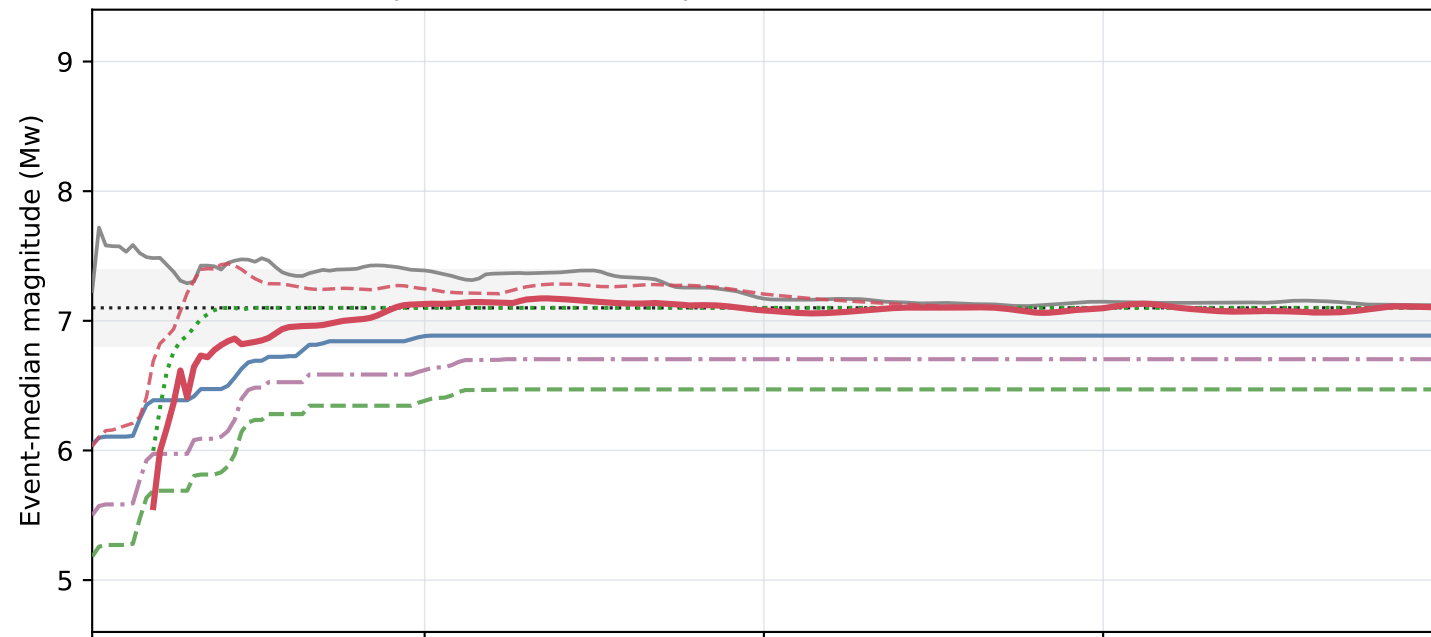
A. Anchorage2018 | catalog Mw 7.10 | 8 stations
