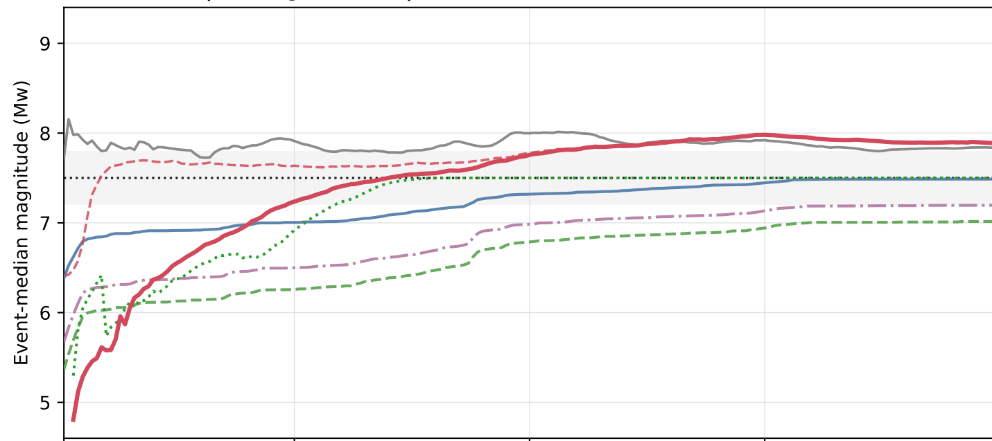
C. Noto2024 | catalog Mw 7.50 | 397 stations
