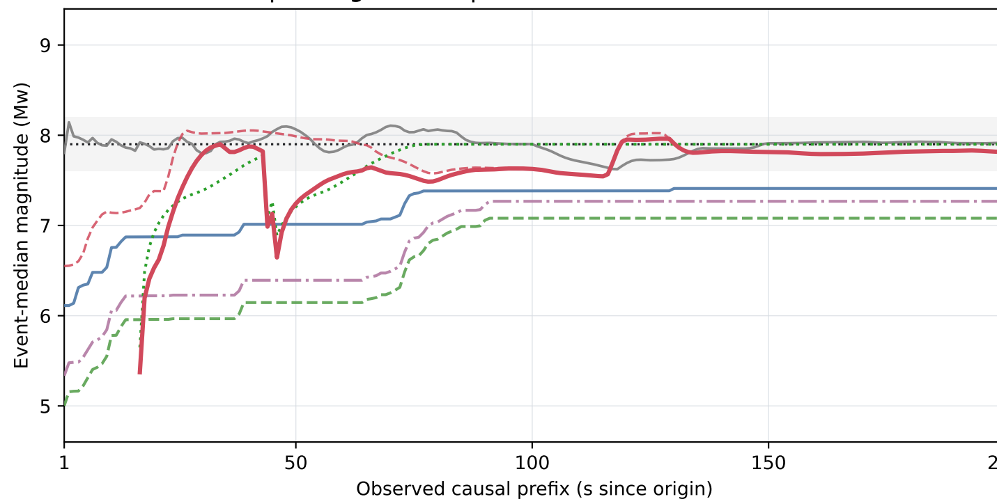
E. RatIslands2014 | catalog Mw 7.90 | 3 stations
