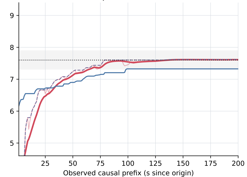
F. SandPoint2020 | Mw 7.60
