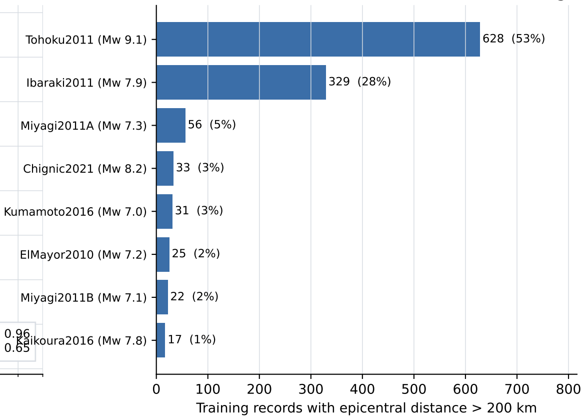
C. Who teaches the far field? (1183 of 1798 training records)
