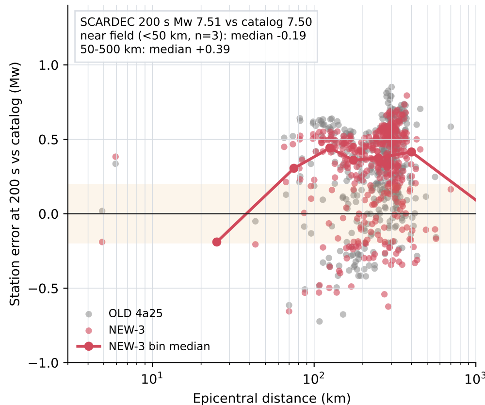
A. Noto2024: 200 s station error vs distance (397 stations)
