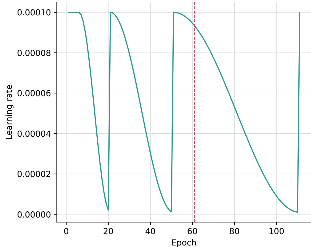
C. Warm-restart schedule
