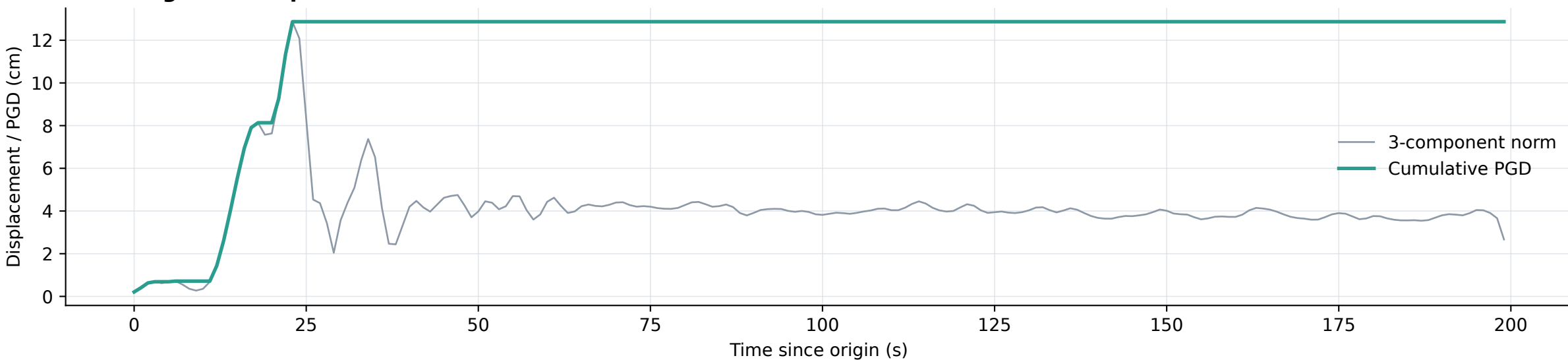
C. Seed-73 endpoint estimates; station P616 = 6.94 Mw
