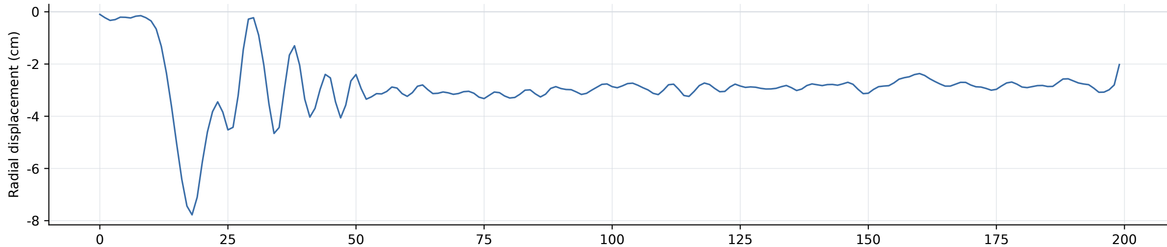
B. Peak ground displacement
