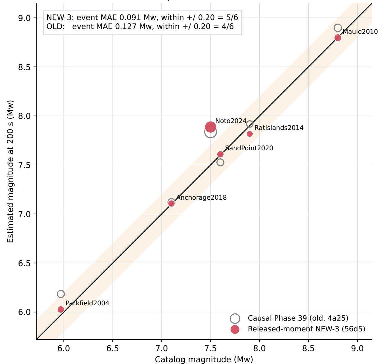
B. Validation (6 events) | marker size = station count
