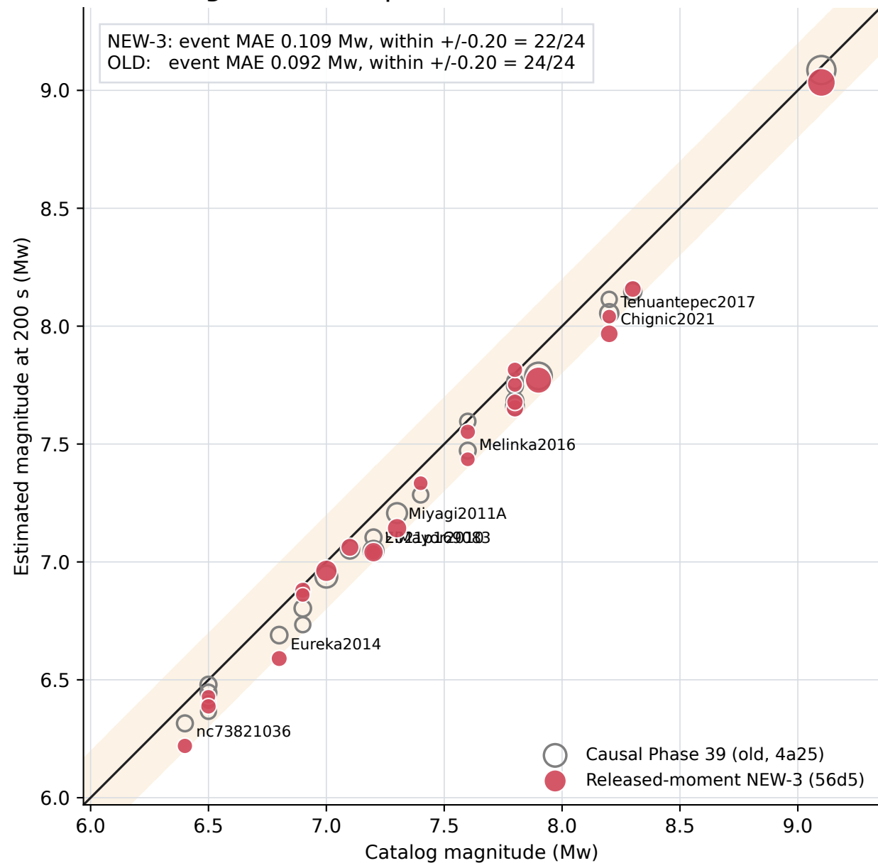
A. Training (24 events) | marker size = station count
