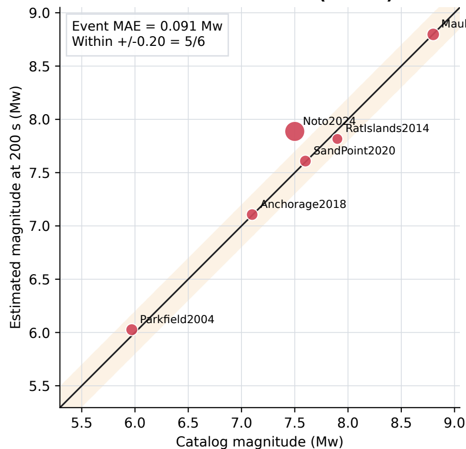
A. Released-moment model (NEW-3)
