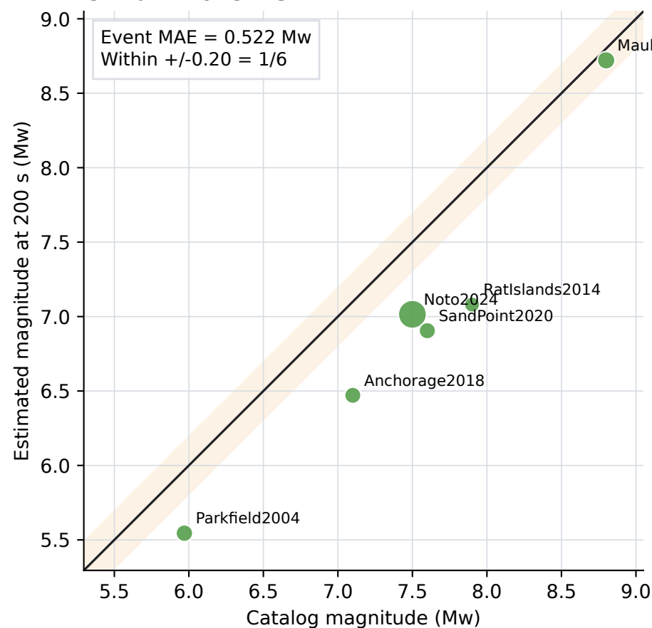
C. Ruhl 2019 PGD
