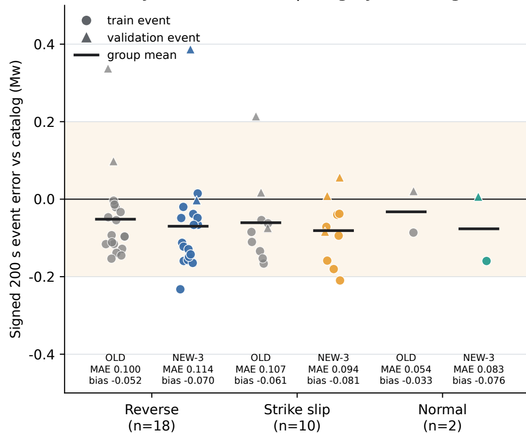
A. Error by focal mechanism | left grey = OLD, right = NEW-3
