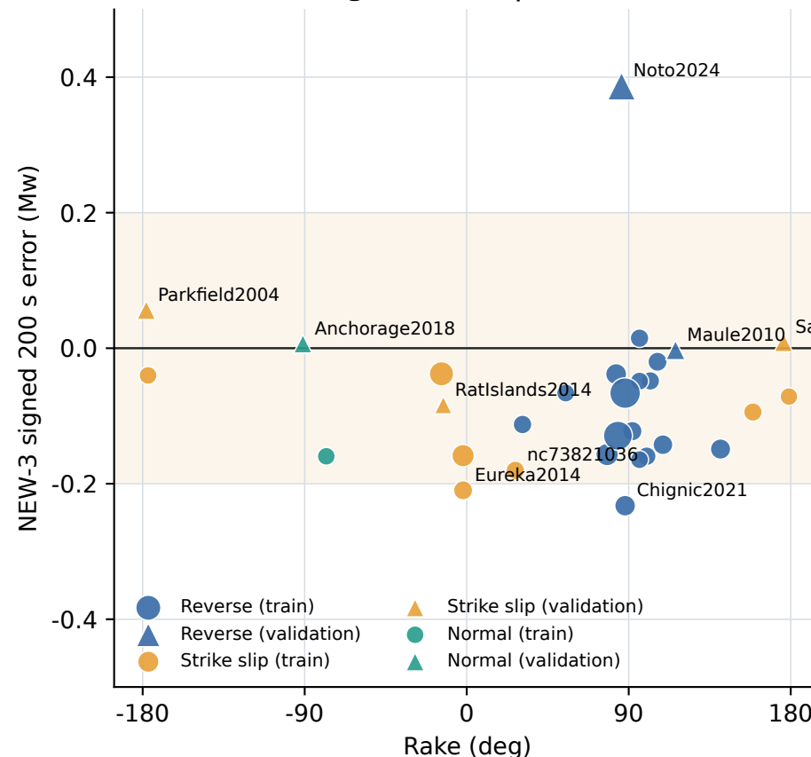
B. NEW-3 error against rake | size = station count
