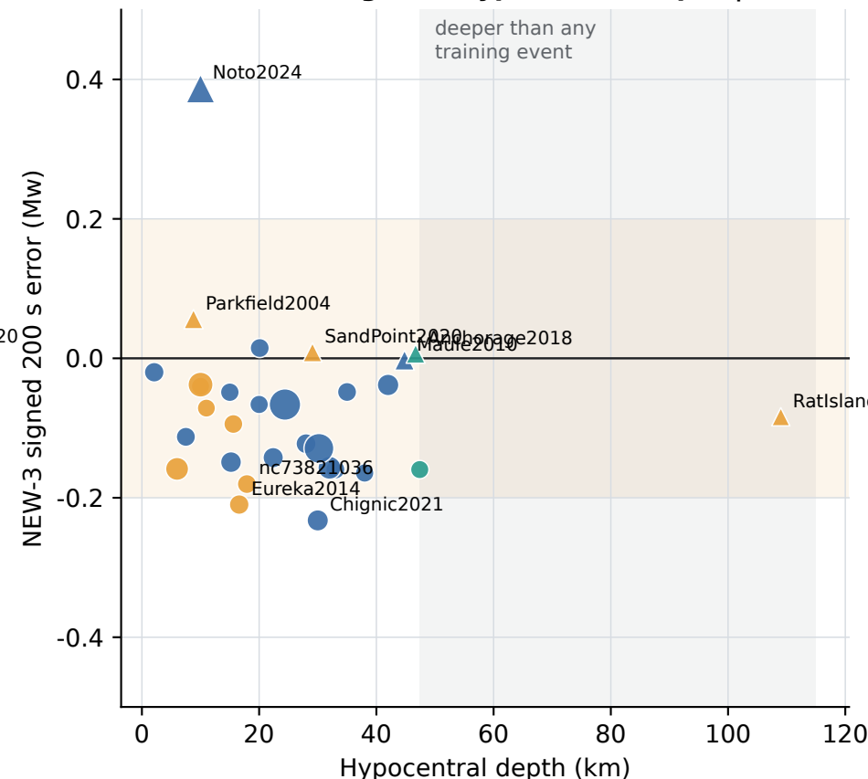
C. NEW-3 error against hypocentral depth | size = station count
