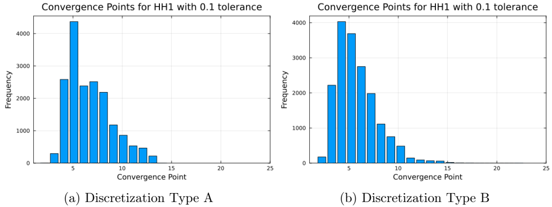
Figure 9.: Convergence point histogram for \epsilon = 0.1 and HH1
