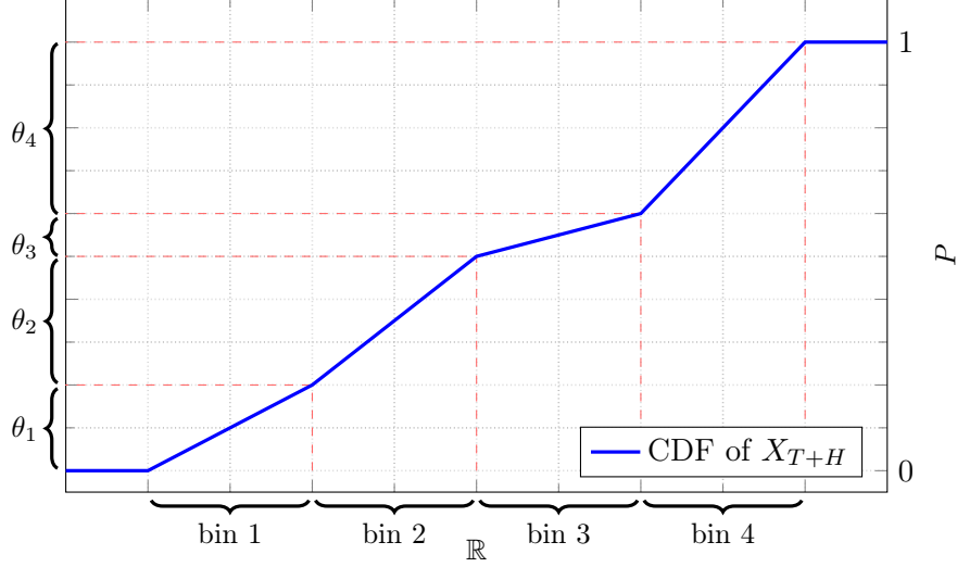
Figure 3.: Continuation of the distribution vector \theta with four exemplary bins.
