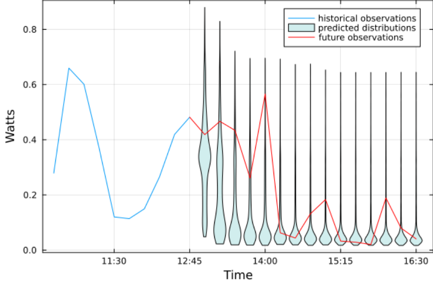
Figure 8.: Example of a typical situation of a multi-step-ahead distribution forecast. Given the historic observation, a distribution forecast is computed for each time instance in the future illustrated by the multiple violin plots. Additionally, the true realization of the future time instances were added to the plot afterwards. Examining the shape of the single distributions, the convergence is visible. From time instance 14:00 onward, the violins do not change significantly and from 15:15 onward, they are visually not differentiable.
