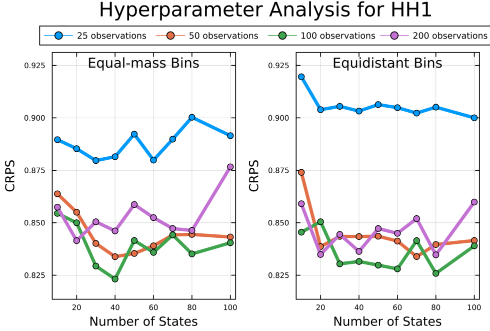
Figure 5.: Representative graph of the hyperparameter analysis of HH1. The left graph displays the results for discretization type A with equal-mass bins, while the graph on the right side shows the results for discretization type B with equidistant bins. The optimal models are chosen by the minimal mean-CRPS value, which is for discretization type A the model with 100 observations and 40 hidden states and for discretization type B the model with 100 observations and 80 hidden states.
