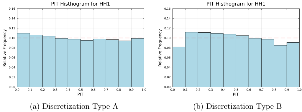
Figure 7.: Representative PIT histograms for HH1
