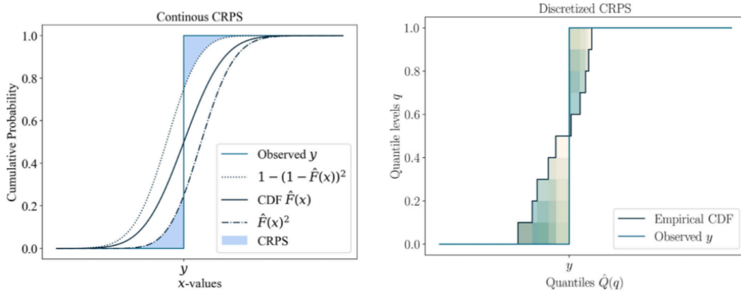
Figure 2.: Graphical example of the continuous and discretized CRPS, reproduced from Botman, Lago, Becker, Vanthournout, and Moor [3]
