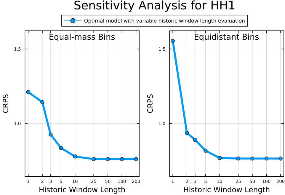
Figure 6.: Representative figure of the result of the sensitivity analysis for HH1.
