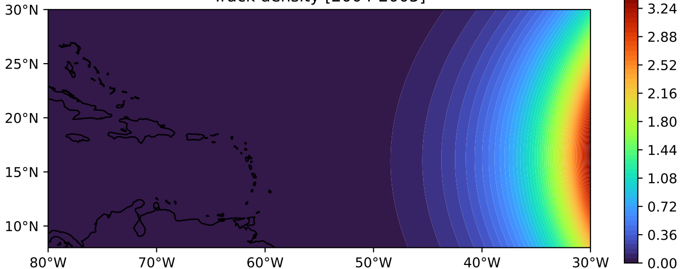
Track density [2004-2005]
