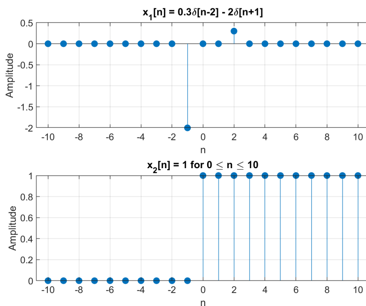
Figure 10: Discrete-time signals representation using subplot
