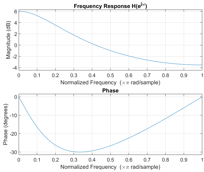
Figure 13: Frequency response H(e^{j\omega})
