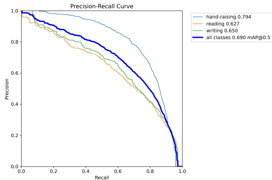
BAC-SSM-YOLO - PR curve
