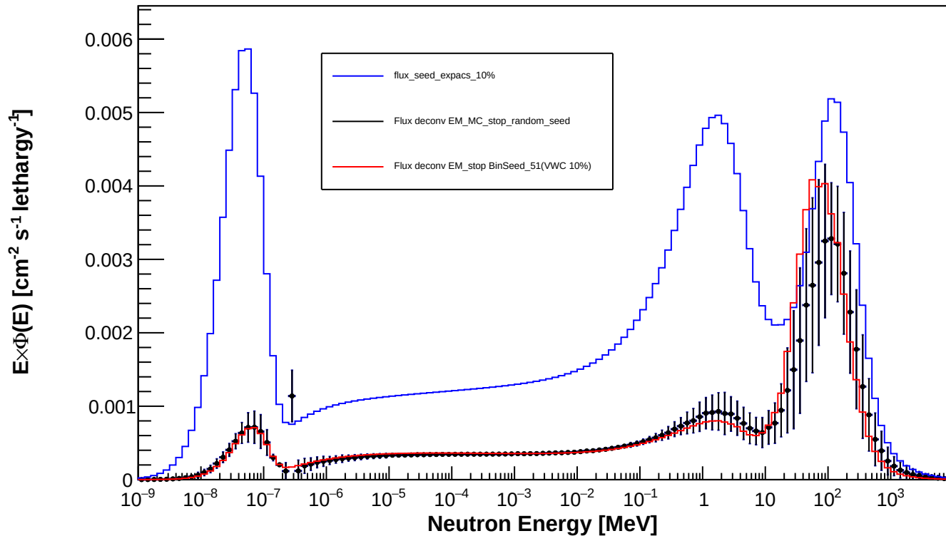
Spectrum_LCO_Event_112_timegrid_15_ndet_11_Random_Seed
