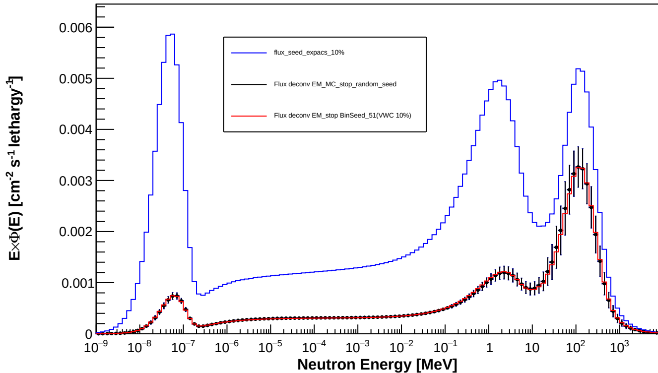
Spectrum_LCO_Event_115_timegrid_15_ndet_11_Random_Seed
