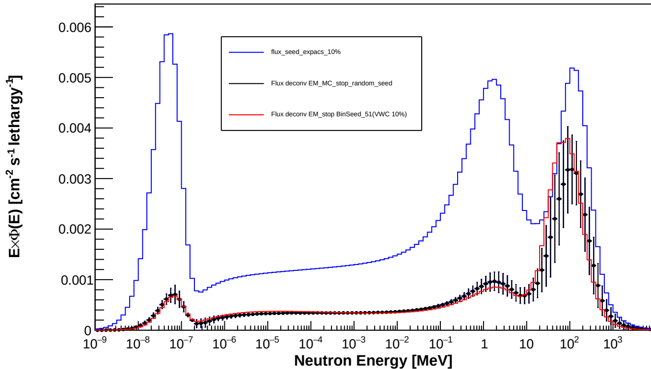
Spectrum_LCO_Event_126_timegrid_15_ndet_11_Random_Seed
